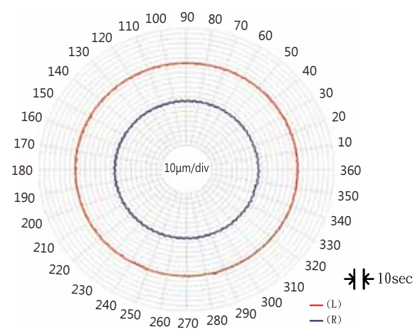
Suface contact and pitch error testing for worm gear system.
